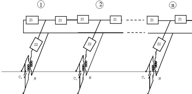
Figure 1. Equivalent circuit representation of a stack with the mechanical ports of each equivalent circuit representing a layer connected in series and n electrical ports in parallel. For Stacks with aspect ratios Length/width < 5 elastic constants are effective.
