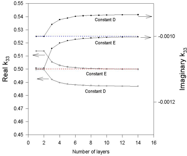
Figure 3. The electromechanical coupling constant k_{33} determined using Smits' method with the impedance equations determined from constant D and constant E elastic boundary conditions. Dotted lines are the real (bottom) and imaginary (top) parts of the input k_{33} .
