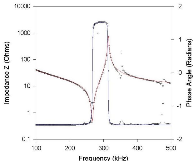
Figure 6. The impedance spectra of a Morgan Matroc stack and the fit (lines) to the spectra (symbols) using the modified Levenberg Marquardt non-linear regression routine.
