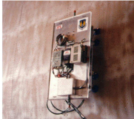
Figure 3: MACS crawling on the C-5 aircraft [Bar -Cohen, et al, 1999].
